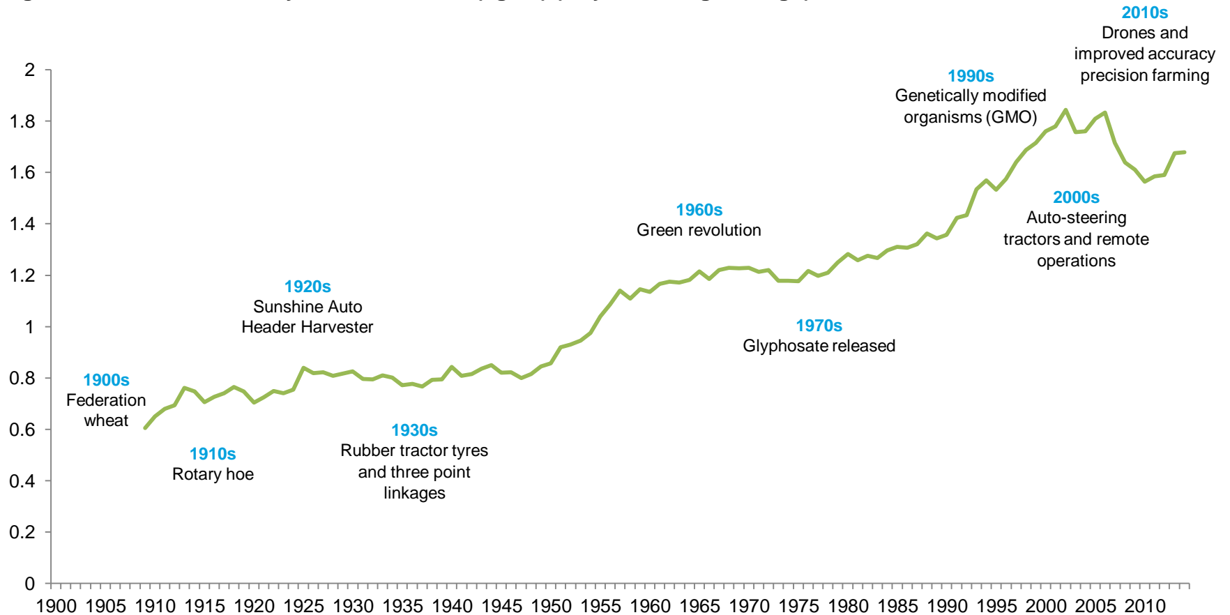
Figure 1: Australian wheat yields: 1905-2014 (kg/ha) (10 year rolling average)
