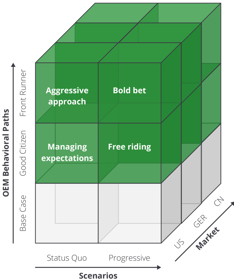
Fig. 3 – Pathway to net-zero model structure
