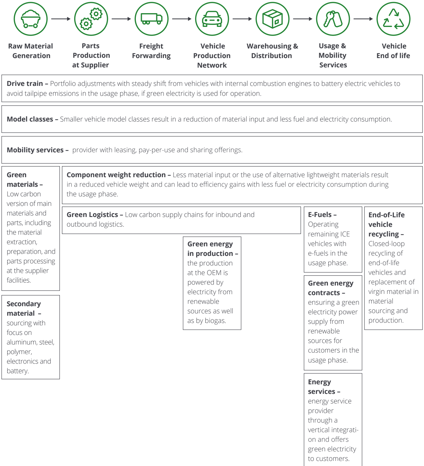
Fig. 6 – Main decarbonization levers across the value chain
